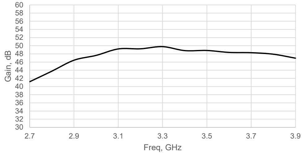
Gain 2.7GHz to 3.9GHz
