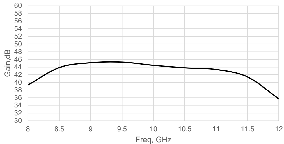
Gain 8GHz to 12GHz
