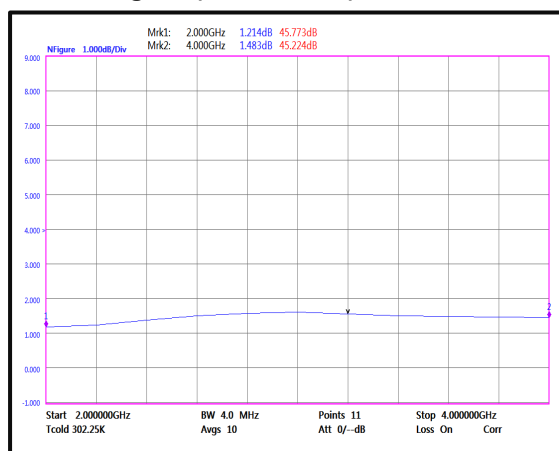
Noise Figure (2GHz-4GHz)
