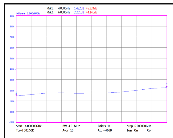
Noise Figure (4GHz-6GHz)
