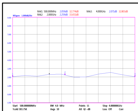
Noise Figure (500MHz-4GHz)
