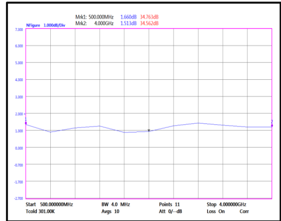
Noise Figure(0.5GHz-4GHz)
