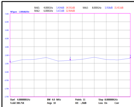
Noise Figure(4GHz-8GHz)
