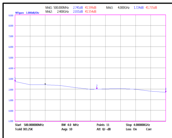
Noise Figure(0.5-4GHz)
