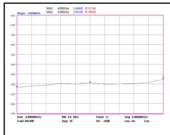
Noise Figure(4-6GHz)
