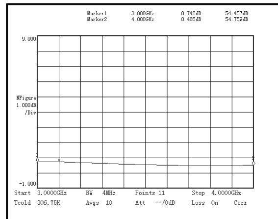
Noise Figure(3-4GHz)
