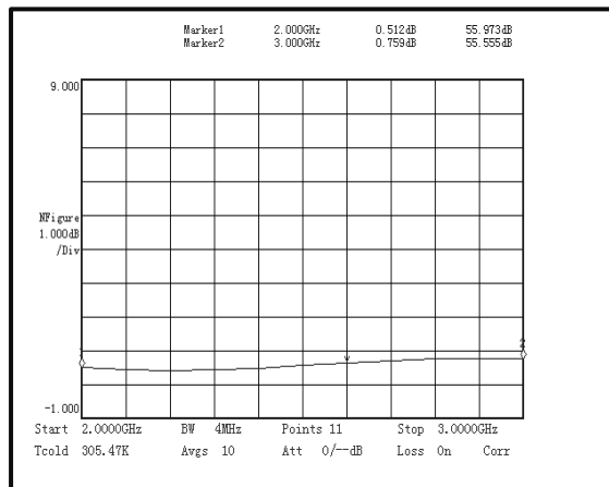
Noise Figure(2-3GHz)
