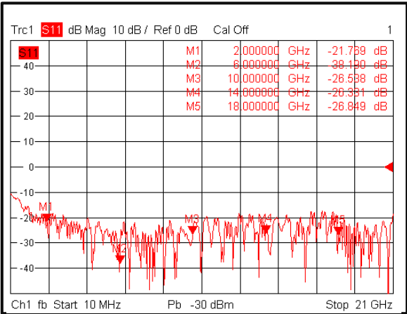
Input Return Loss vs Frequency @+25°C
