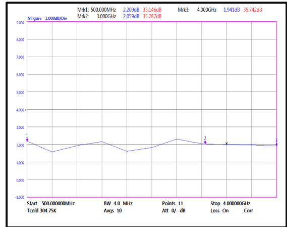
Noise Figure(0.5-4GHz)
