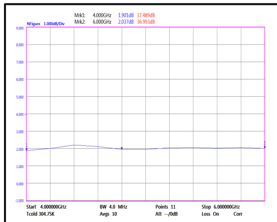
Noise Figure(4-6GHz)
