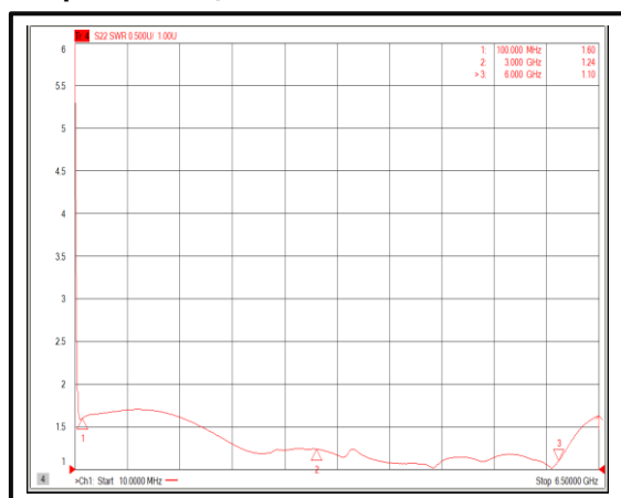
Output VSWR@+25°C
