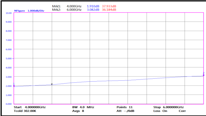
Noise Figure(4GHz-6GHz)
