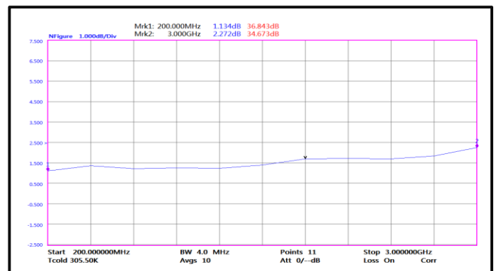
Noise Figure(0.2GHz-3GHz)
