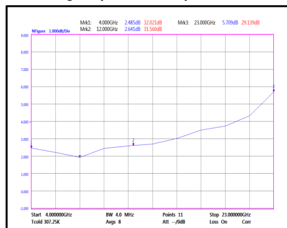
Noise Figure (4GHz-23GHz)
