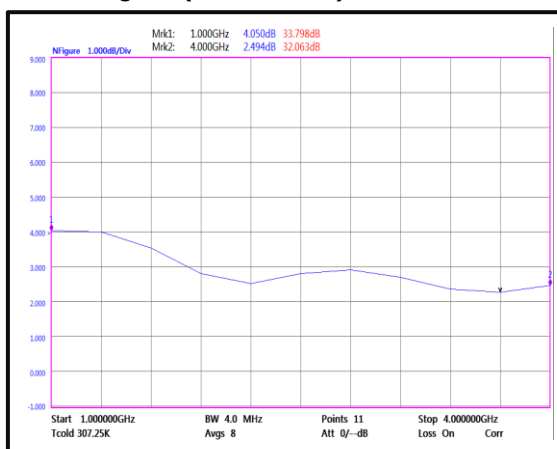
Noise Figure (1GHz-4GHz)
