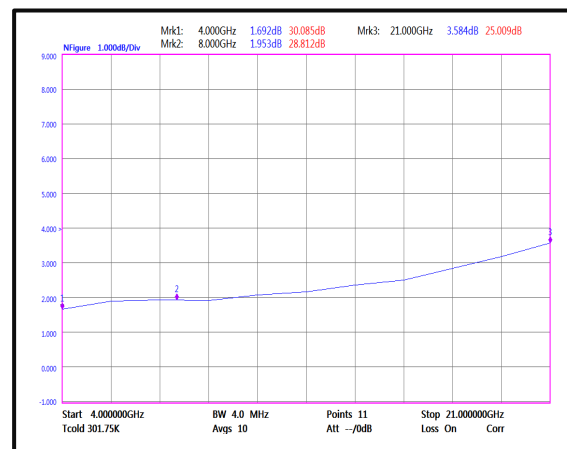
Noise Figure(4-21GHz)
