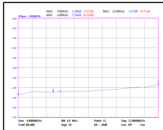
Noise Figure (4-12GHz)
