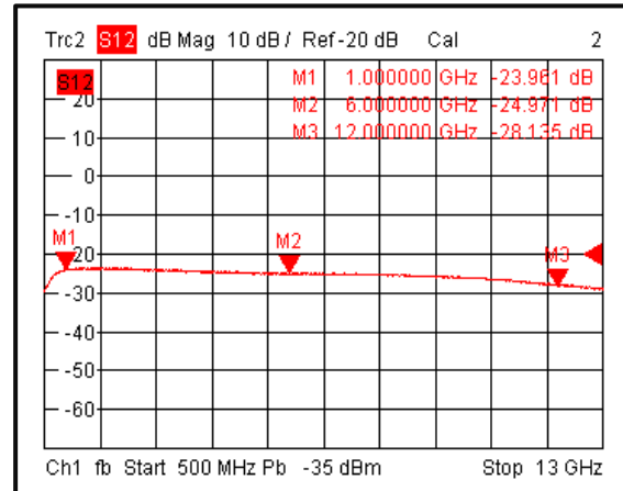
Isolation @-45°C
