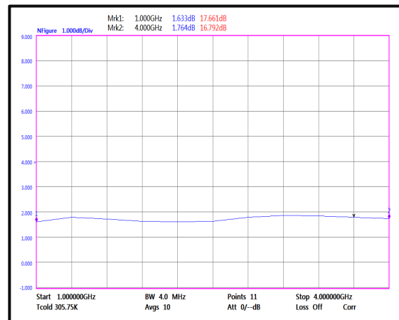
Noise Figure (1-4GHz)
