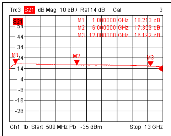
Gain @-45°C
