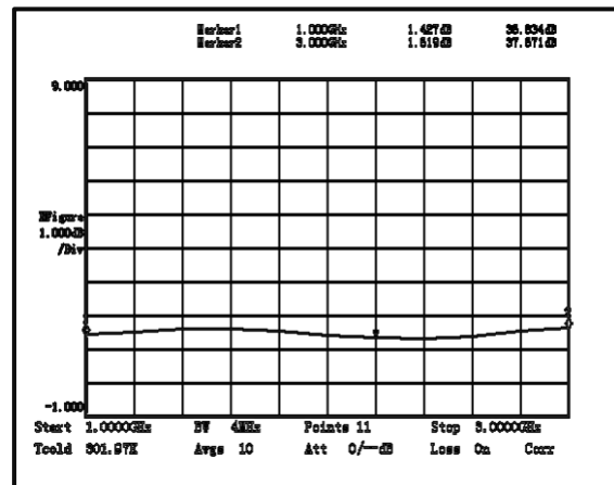
Noise Figure (1-3GHz)
