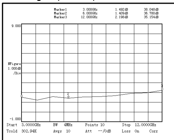
Noise Figure (3-12GHz)
