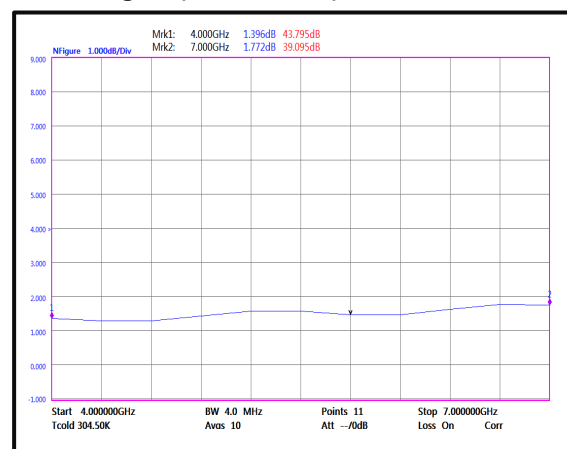
Noise Figure(4GHz-7GHz)
