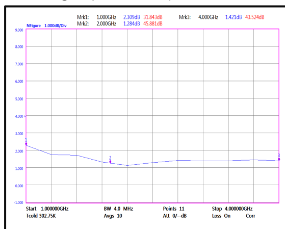
Noise Figure(1GHz-4GHz)
