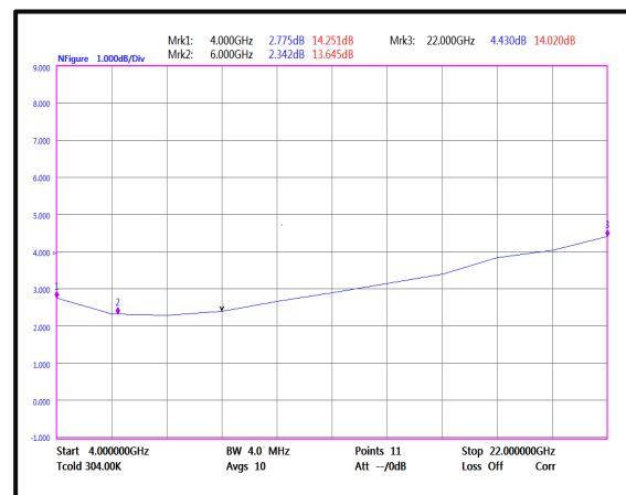
Noise Figure(4-22GHz)
