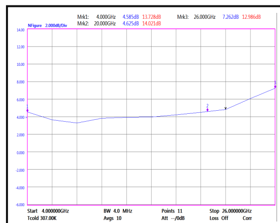
Noise Figure(4-26GHz)
