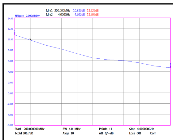
Noise Figure(0.2-4GHz)
