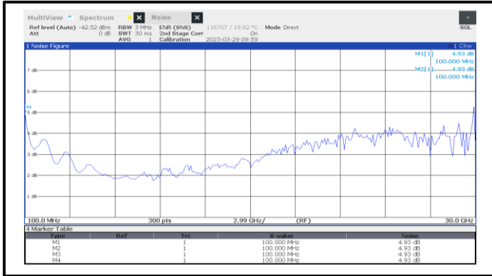
Noise Figure(0.1GHz-30GHz)
