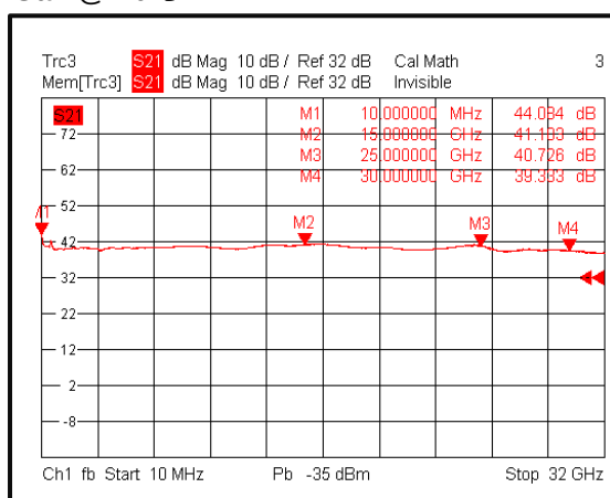
Gain@-40°C
