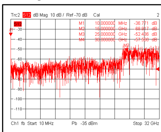
Isolation@-40°C
