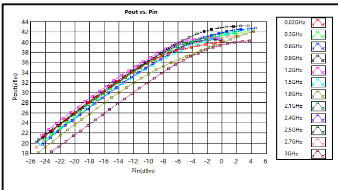
Pout vs. Pin CW
