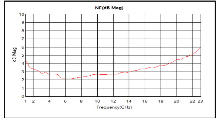
Noise Figure
