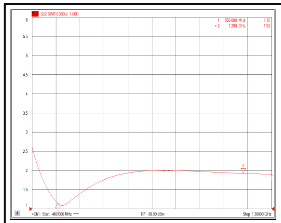
Output VSWR@+85°C (+5V)
