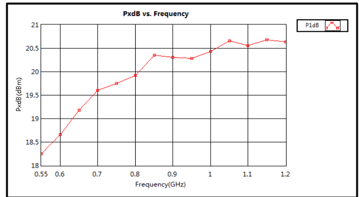
P1dB vs. Frequency (+5V)
