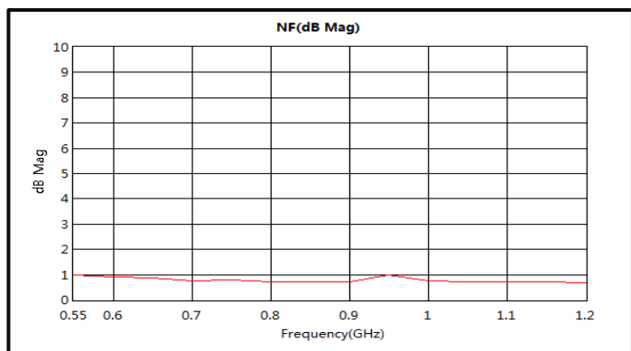
Noise Figure (+3V)
