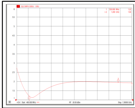
Output VSWR@+25°C (+5V)
