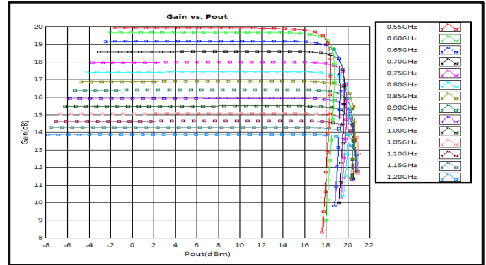
Gain vs. Output Power (+5V)
