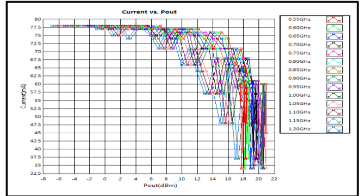
Current vs. Pout (+5V)
