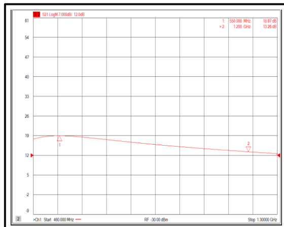
Gain@-40°C (+3V)
