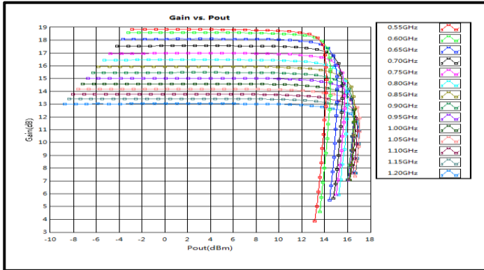
Gain vs. Output Power (+3V)
