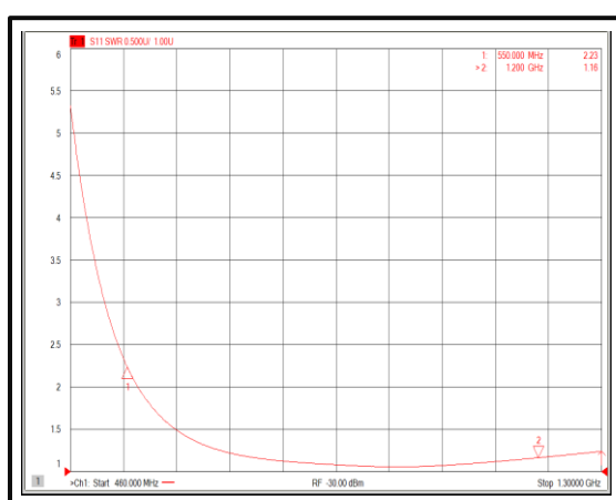
Input VSWR@+85°C (+3V)
