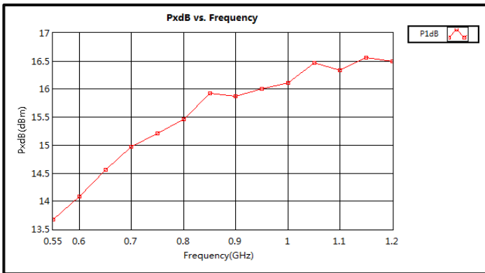
P1dB vs. Frequency (+3V)
