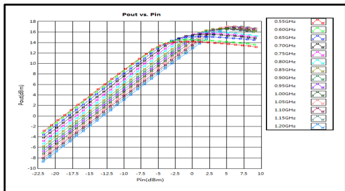
Pout vs. Pin (+3V)
