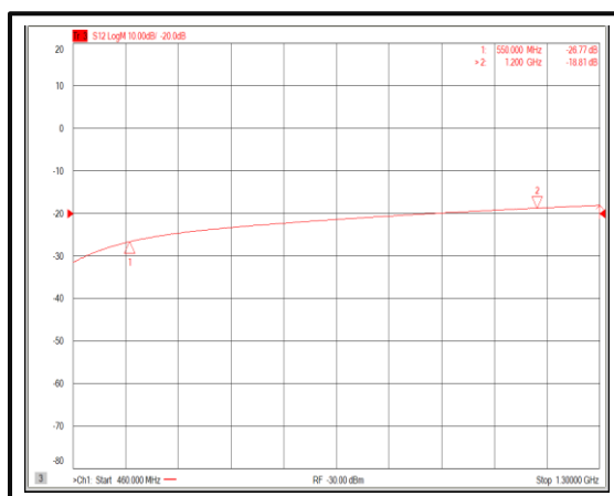
Isolation@-40°C (+5V)
