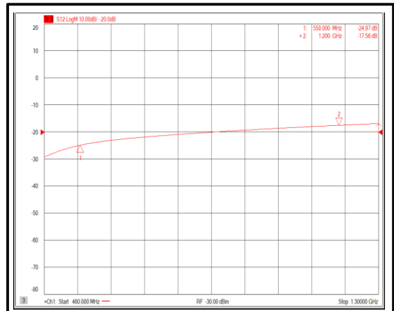
Isolation@-40°C (+3V)
