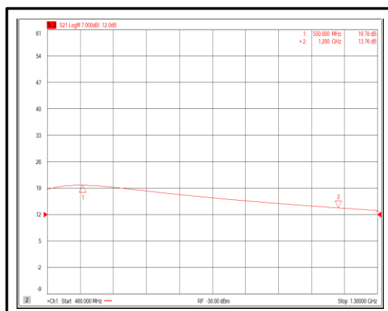
Gain@+85°C (+5V)
