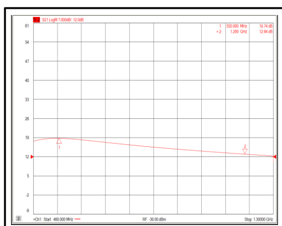
Gain@+85°C (+3V)
