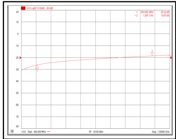
Isolation@+25°C (+5V)
