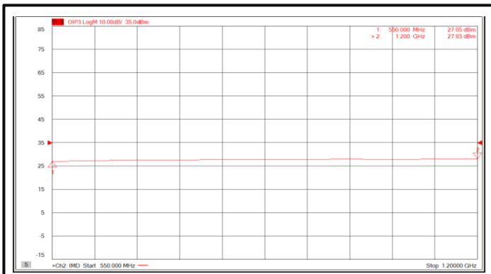
Output Third Order Intercept (OIP3) (+3V)
