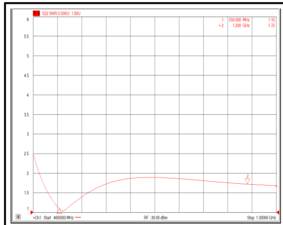
Output VSWR@-40°C (+3V)
