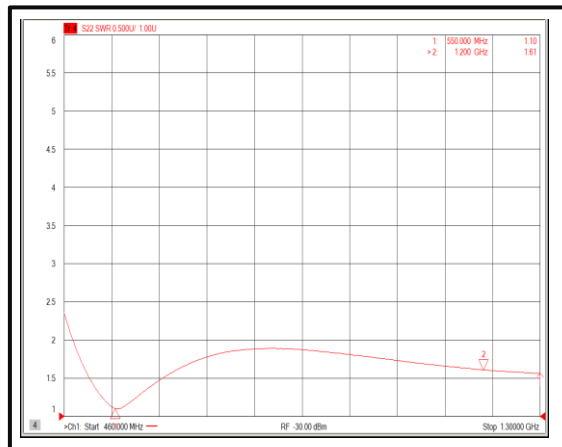
Output VSWR@+85°C (+3V)
