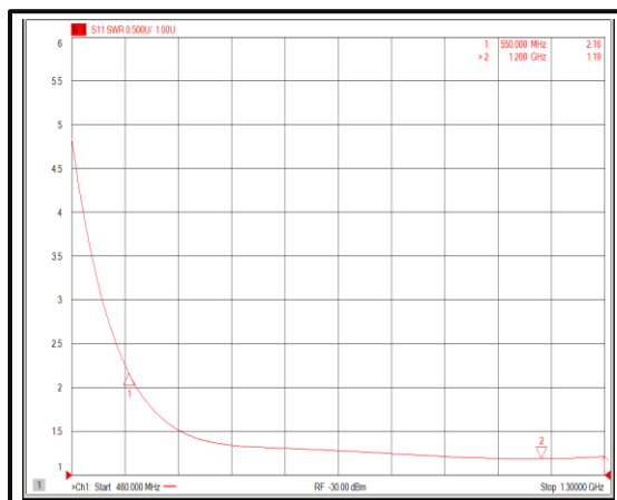
Input VSWR@+25°C (+5V)
