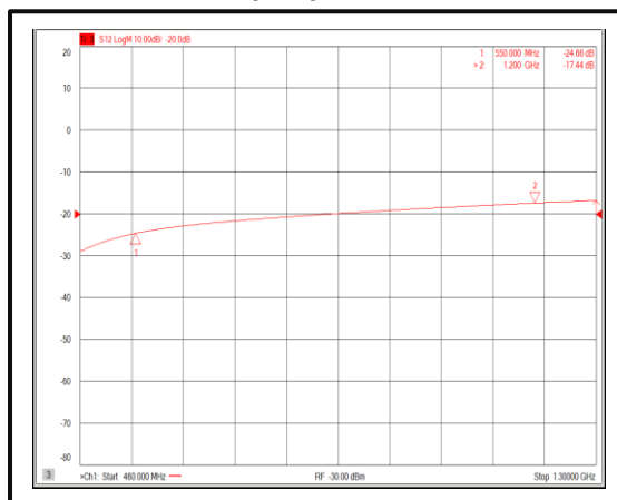
Isolation@+25°C (+3V)
