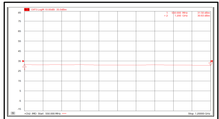
Output Third Order Intercept (OIP3) (+5V)
