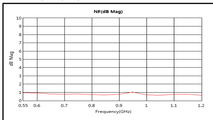
Noise Figure (+5V)
