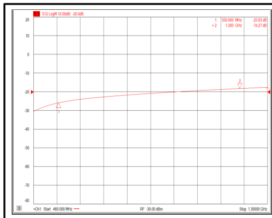
Isolation@+85°C (+5V)
