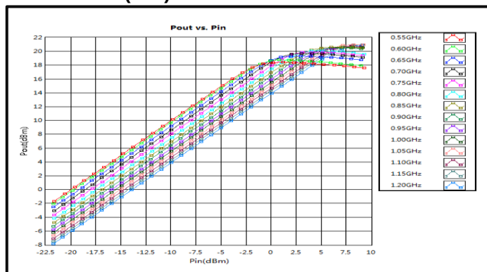
Pout vs. Pin (+5V)
