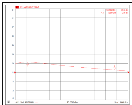
Gain@+25°C (+5V)
