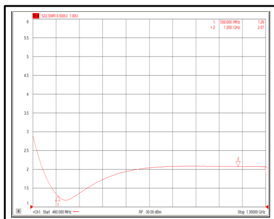
Output VSWR@-40°C (+5V)
