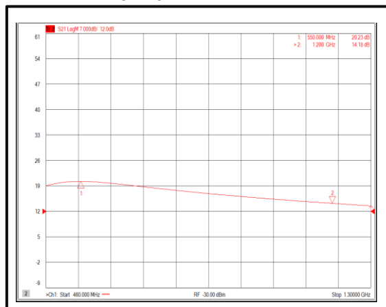
Gain@-40°C (+5V)
