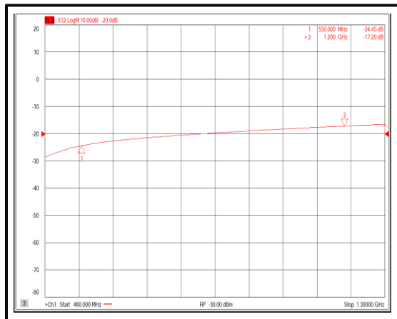
Isolation@+85°C (+3V)
