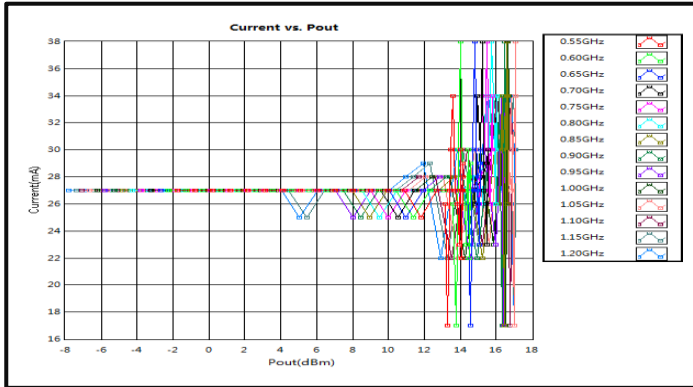
Current vs. Pout (+3V)
