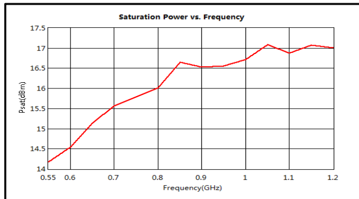
Saturation Power vs. Frequency (+3V)
