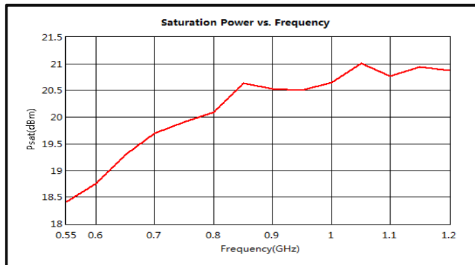
Saturation Power vs. Frequency (+5V)
