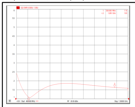
Output VSWR@+25°C (+3V)
