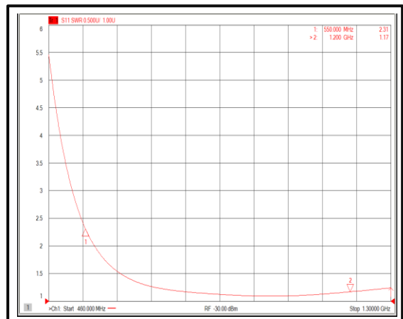
Input VSWR@-40°C (+3V)
