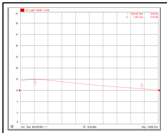
Gain@+25°C (+3V)
