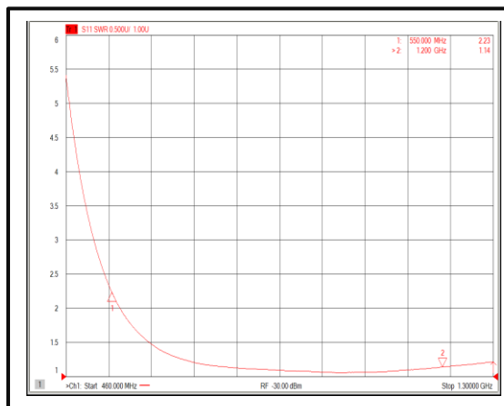
Input VSWR@+25°C (+3V)
