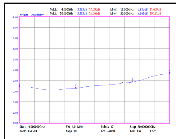
Noise Figure(4-20GHz)
