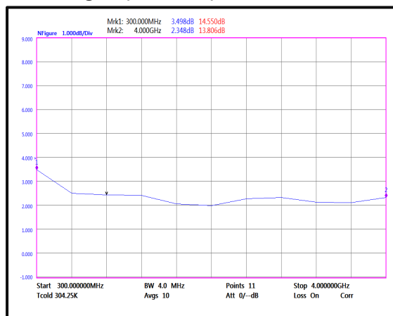
Noise Figure(0.3-4GHz)
