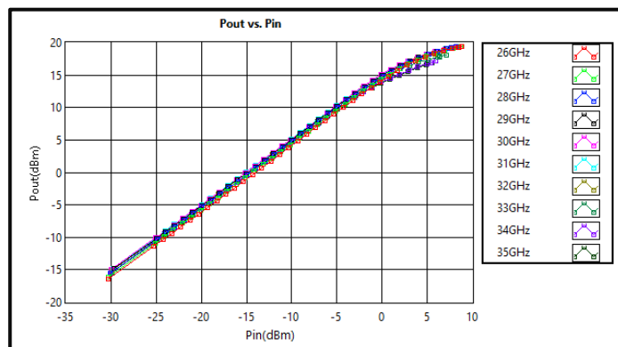
Output vs Input Power @ +25°C
