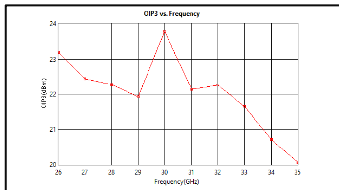
OIP3 vs Frequency @ +25°C
