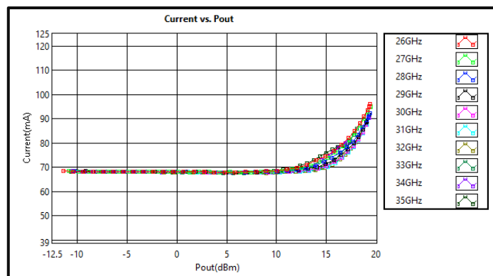
Current vs Output Power (+5VDC) @ +25°C
