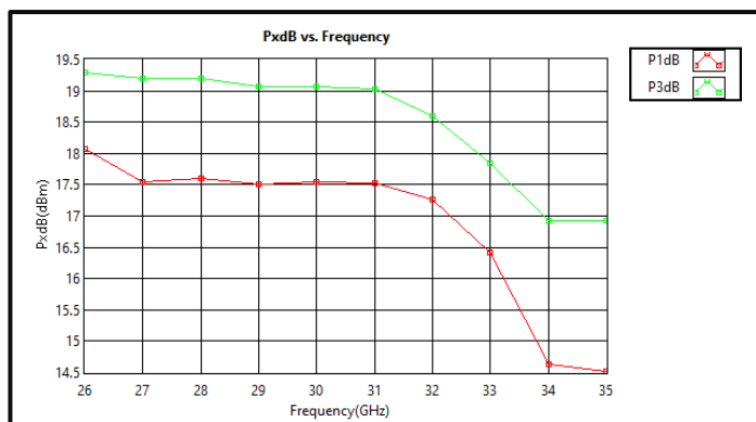
PxdB vs Frequency @ +25°C
