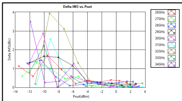
Delta IM3 vs Output Power (+2VDC)
