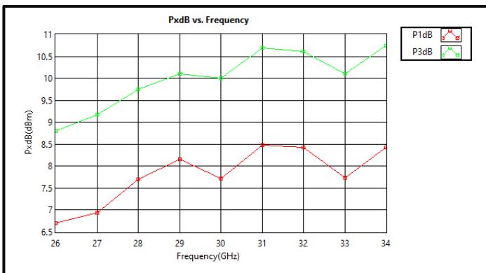
PxdB vs Frequency (+3VDC)
