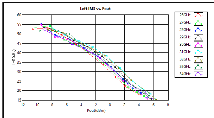
Left IM3 vs Output Power (+3VDC)
