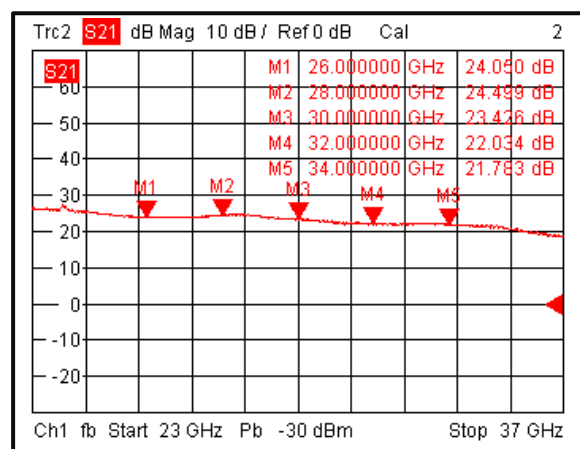
Gain vs. Frequency @-40°C (+2/+3VDC)
