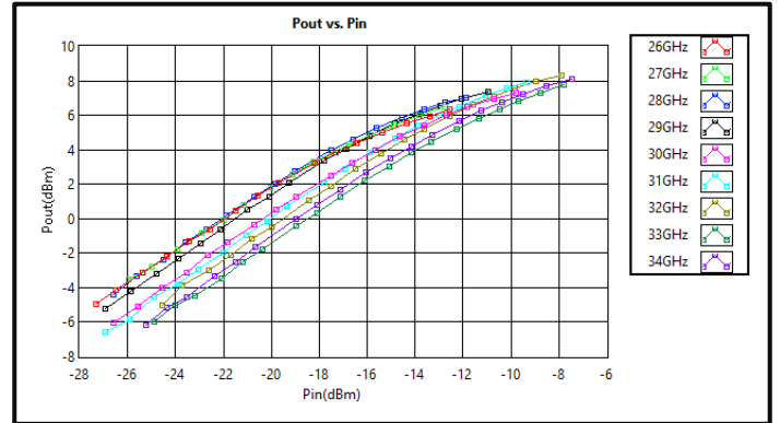
Output vs Input Power (+2VDC)
