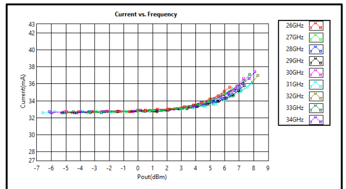
Current vs Output Power (+2VDC)
