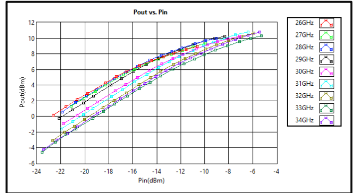
Output vs Input Power (+3VDC)
