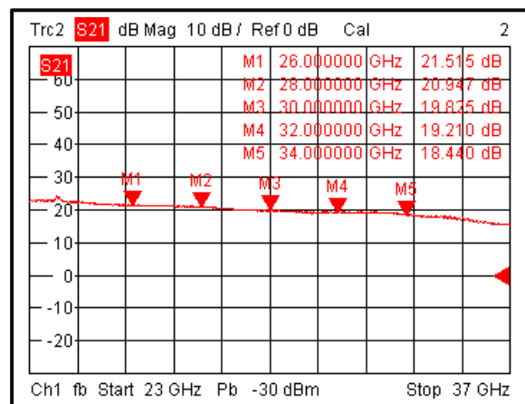
Gain vs. Frequency @+85°C (+2/+3VDC)
