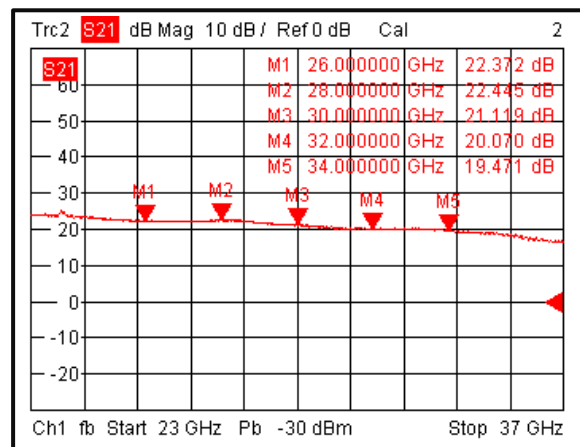
Gain vs. Frequency @+25°C (+2/+3VDC)
