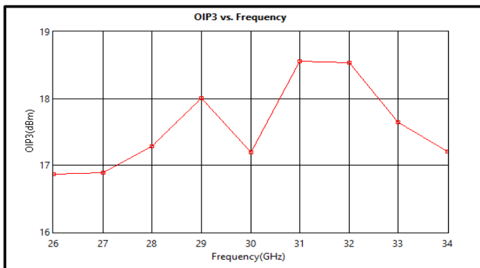
OIP3 vs Frequency (+3VDC)
