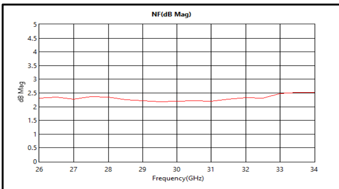
Noise Figure vs Frequency (+2/+3VDC)
