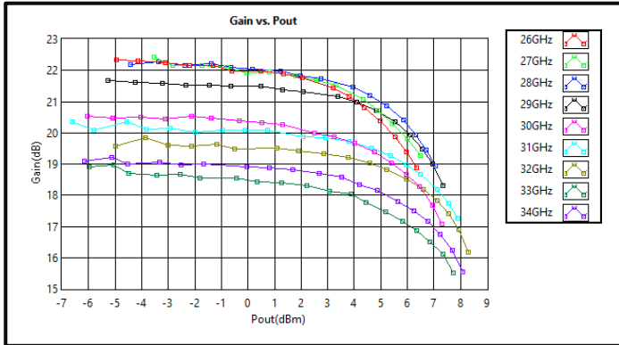
Gain vs Output Power (+2VDC)
