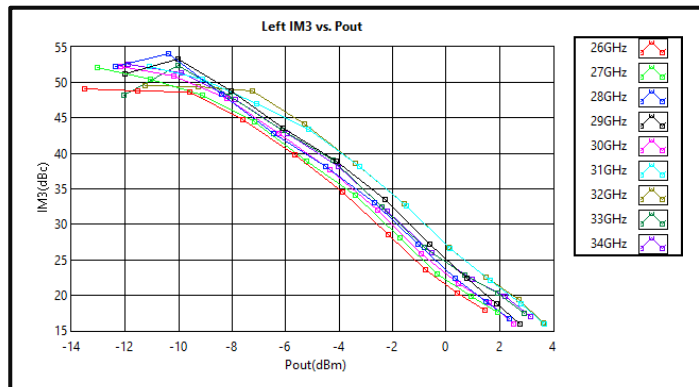
Left IM3 vs Output Power (+2VDC)
