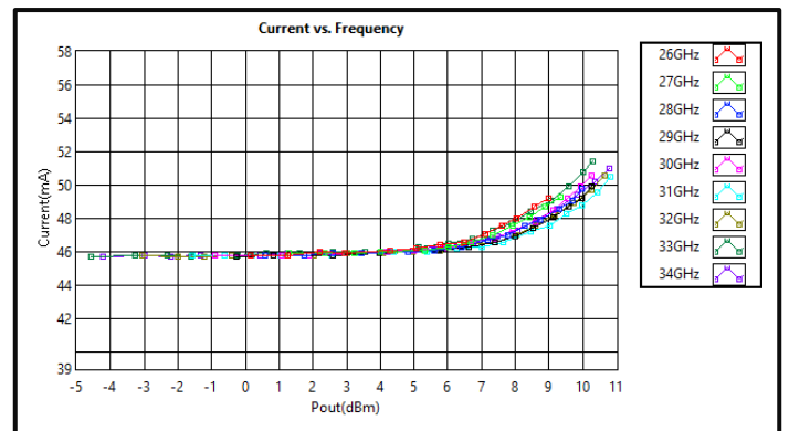
Current vs Output Power (+3VDC)
