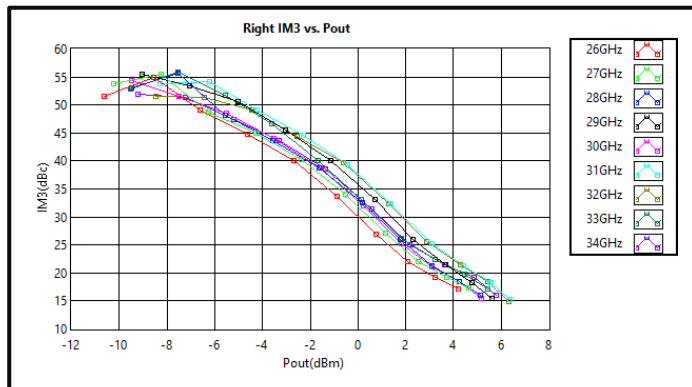
Right IM3 vs Output Power (+3VDC)
