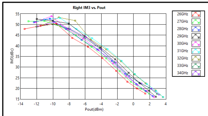
Right IM3 vs Output Power (+2VDC)
