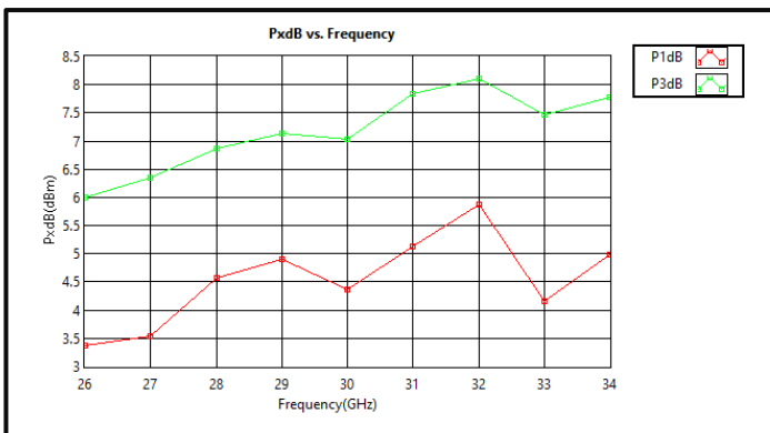
PxdB vs Frequency (+2VDC)
