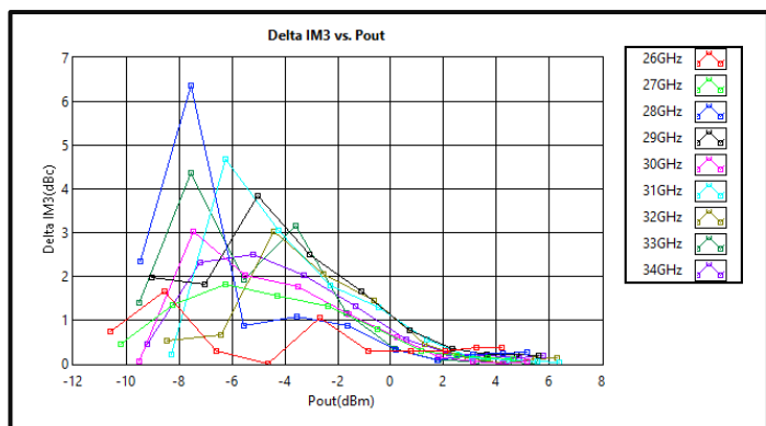
Delta IM3 vs Output Power (+3VDC)
