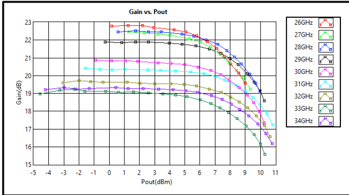
Gain vs Output Power (+3VDC)
