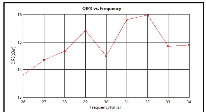
OIP3 vs Frequency (+2VDC)
