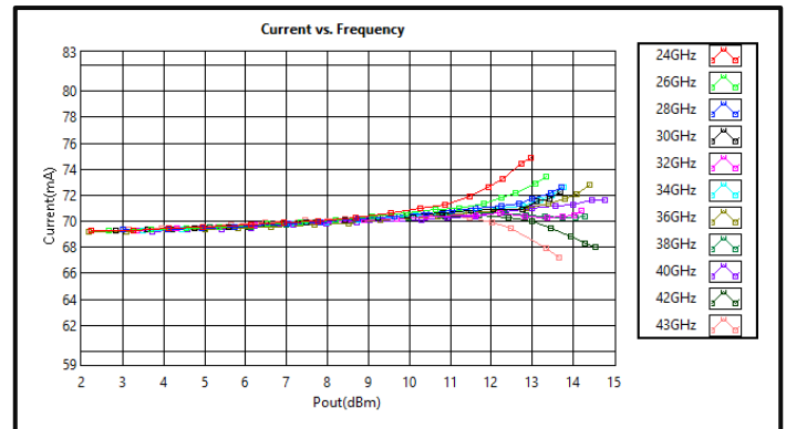
Current vs Output Power (+2.5VDC)
