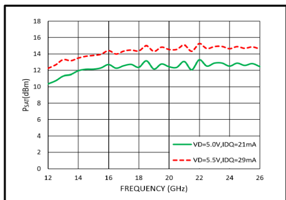
Saturation Power vs. Frequency
