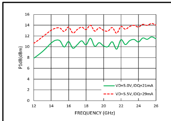
PndB vs. Frequency
