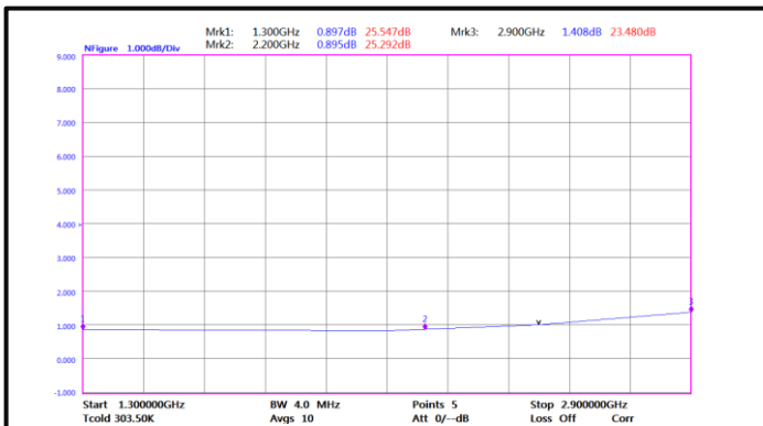
Noise Figure(1-4GHz)
