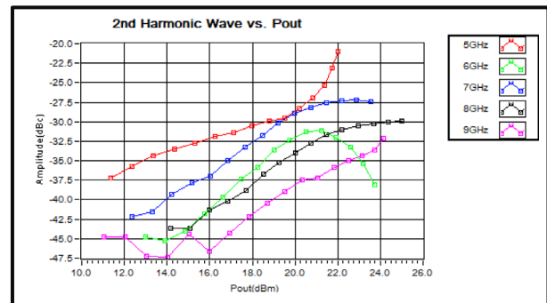
2nd Harmonic Wave Output Power
