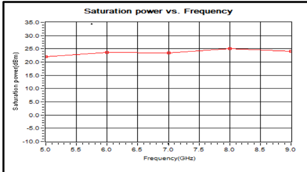
Psat vs. Frequency
