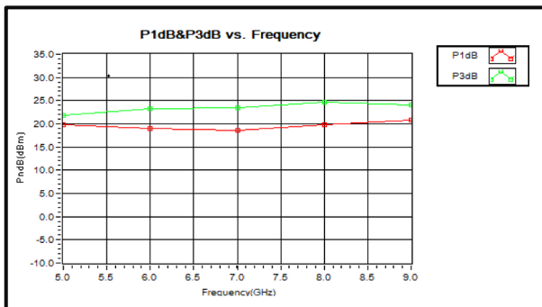
PxdB vs. Frequency
