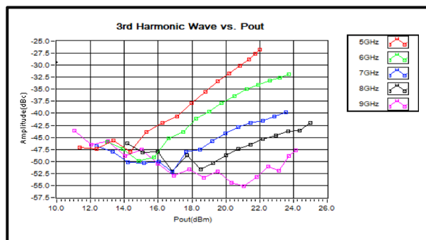
3rd Harmonic Wave Output Power
