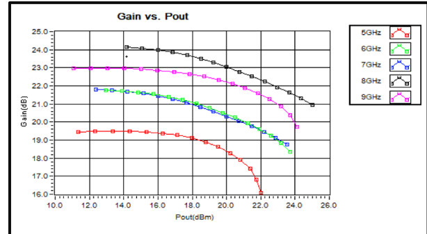
Gain vs. Pout
