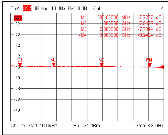
Output Return Loss@-40°C
