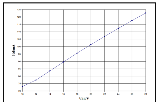
Drain Current vs. Drain Voltage
