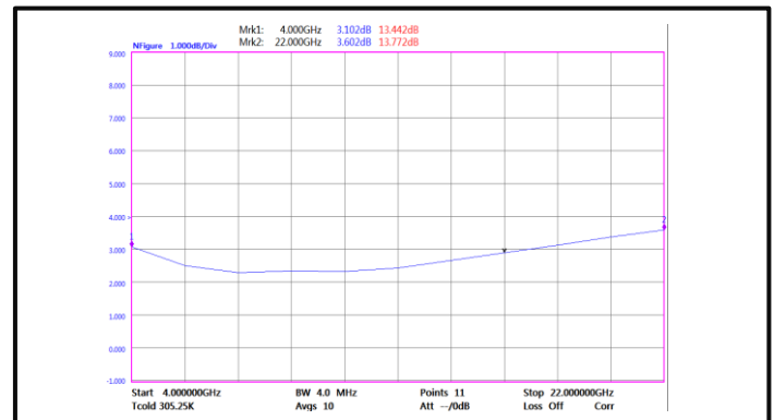
Noise Figure(4GHz-22GHz)
