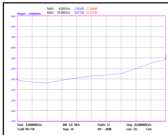
Noise Figure(4GHz-20GHz)
