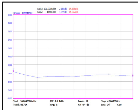
Noise Figure(0.1GHz-4GHz)
