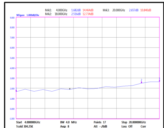
Noise Figure(4GHz-20GHz)
