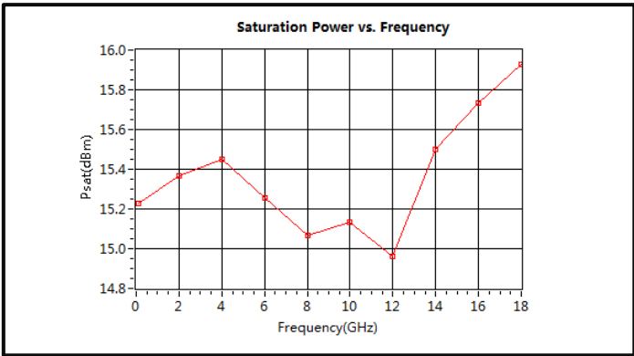
Saturation Power vs. Frequency
