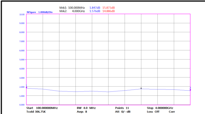
Noise Figure(0.1GHz-4GHz)
