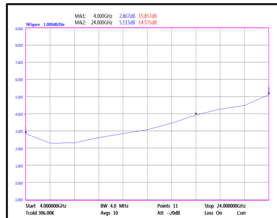
Noise Figure(4-24GHz)
