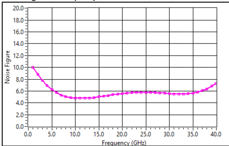
Noise Figure vs. Frequency
