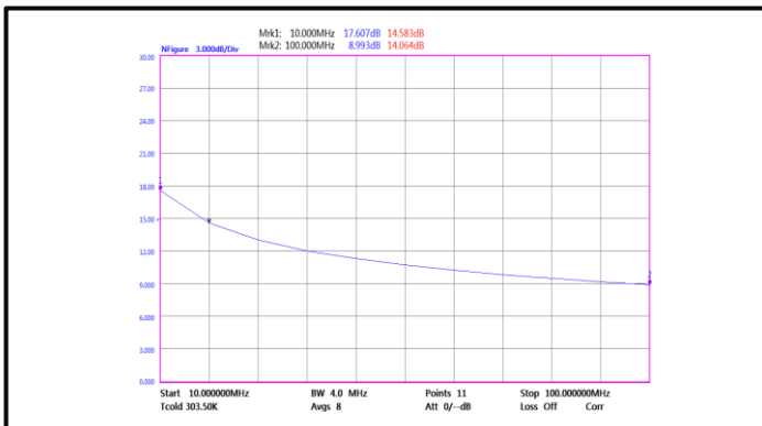
Noise Figure(10MHz-100MHz)
