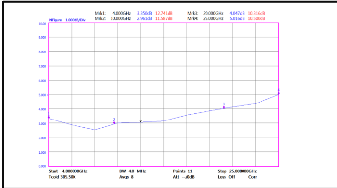
Noise Figure(4GHz-25GHz)
