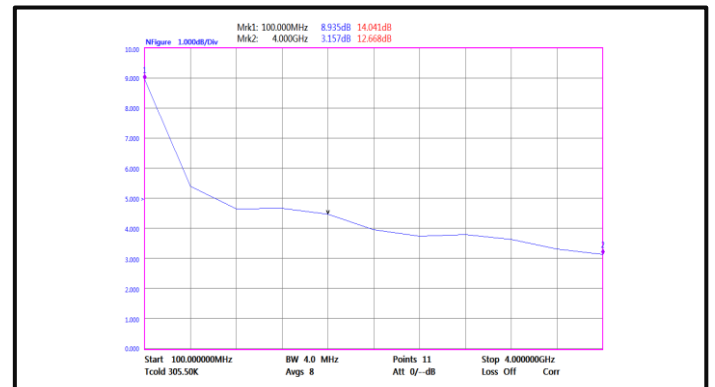
Noise Figure(0.1GHz-4GHz)
