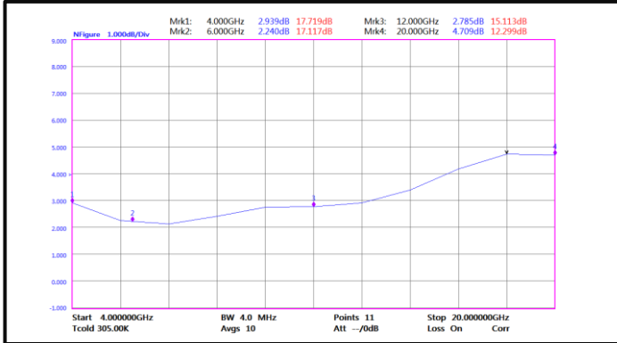
Noise Figure(4GHz-20GHz)
