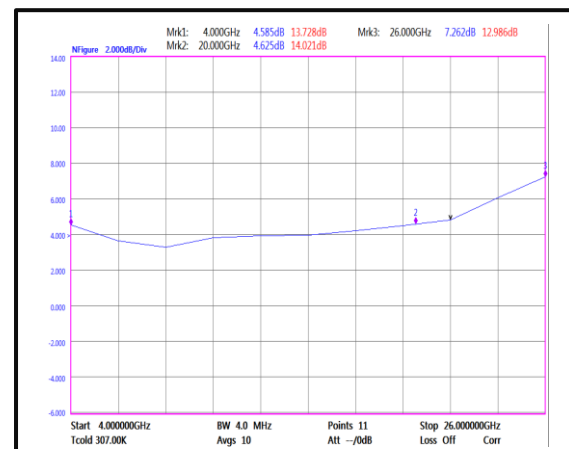
Noise Figure(4-26GHz)
