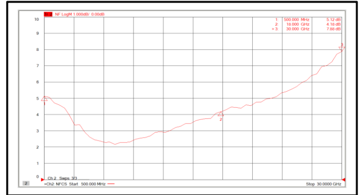
Noise Figure (500MHz-30GHz)
