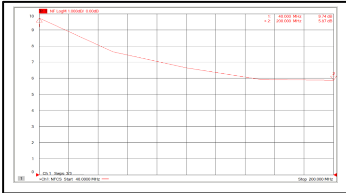
Noise Figure (40MHz-200MHz)
