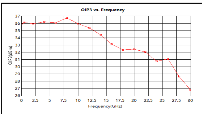
Output Third Order Intercept (OIP3) CW
