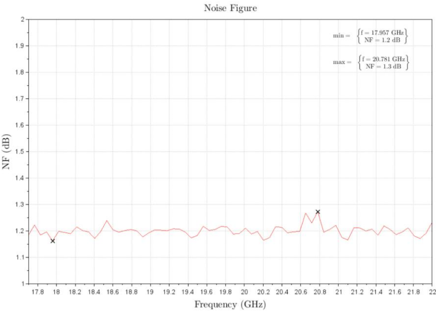
Figure 3: ERZ-LNA-1770-2200-40-1.2 Noise Figure.
