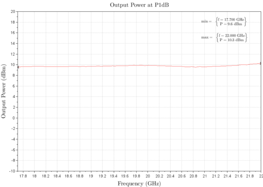
Figure 4: ERZ-LNA-1770-2200-40-1.2 P1dB
