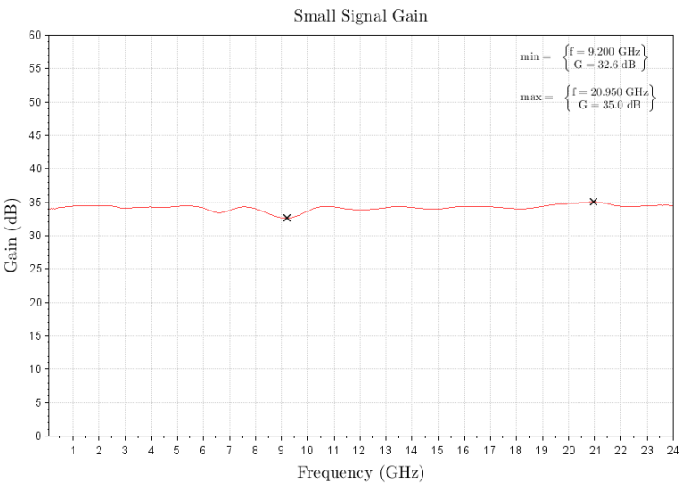
Figure 2: ERZ-LNA-0010-2400-30-4 Small Signal Gain
