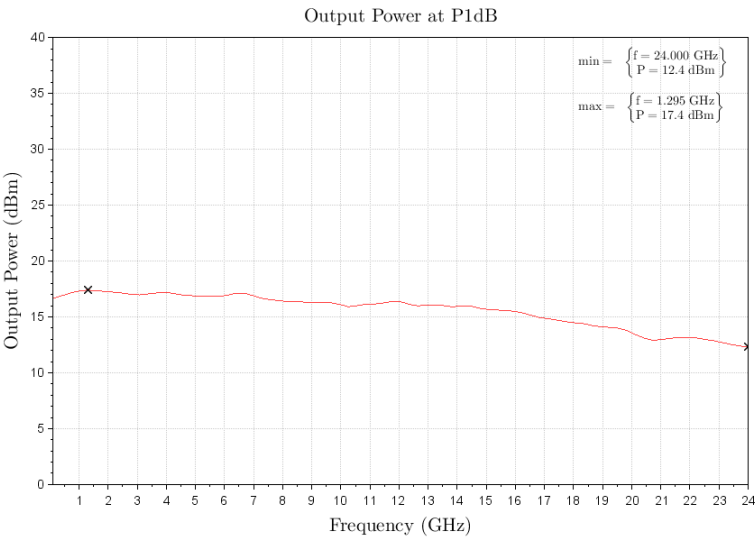
Figure 1: ERZ-LNA-0010-2400-30-4 P1dB
