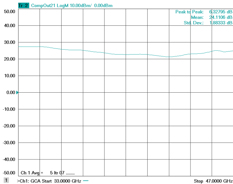
Figure 1: ERZ-HPA-3300-4700-24 P sat
