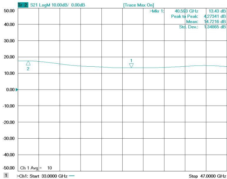
Figure 2: ERZ-HPA-3300-4700-24 Small Signal Gain
