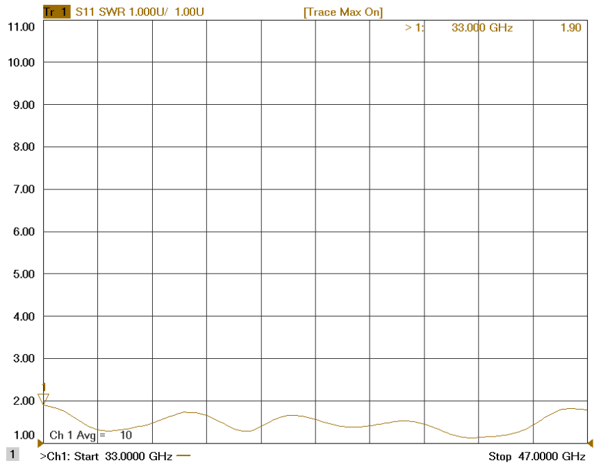
Figure 4: ERZ-HPA-3300-4700-24 Input Matching
