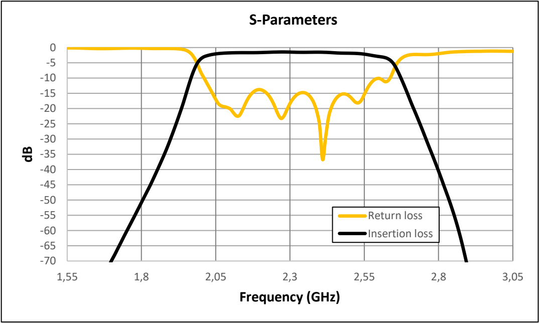
Figure 1:ERZ-BPF-0205-0255-2.2 Insertion & Return loss
