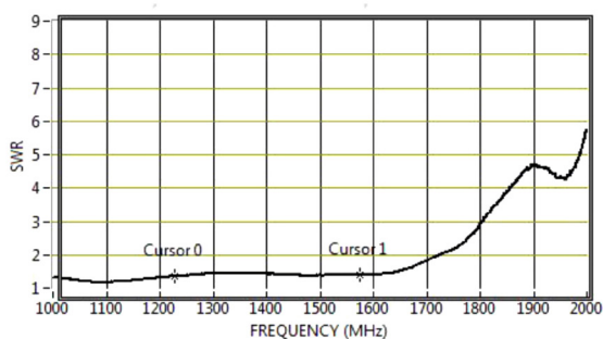
Figure 2-4. Active MS14 Splitter: SWR vs. Frequency
