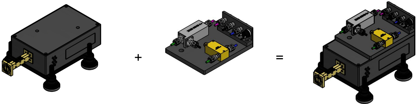
FIGURE 10: PHOTO OF TRIPLEXER (SOLD SEPARATELY) MOUNTING ON RX MODULE. THE RX MODULE WITH -TPLX IS CONFIGURED WITH MOUNTING HOLES ON THE LID.
