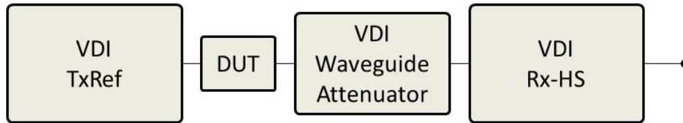
FIGURE 13: BLOCK DIAGRAM OF THE STANDARD OPERATION MODE OF A VDI RX MODULE
