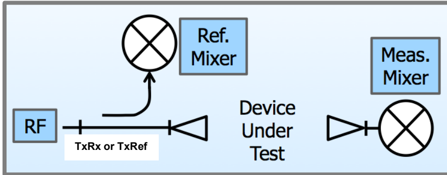
FIGURE 15: A TYPICAL ENHANCED S 21 CONFIGURATION CONSISTS OF ONE HIGH POWER TxREF MODULE ON PORT 1 AND A HIGH SENSITIVITY RX MODULE (Rx-HS) ON PORT 2
