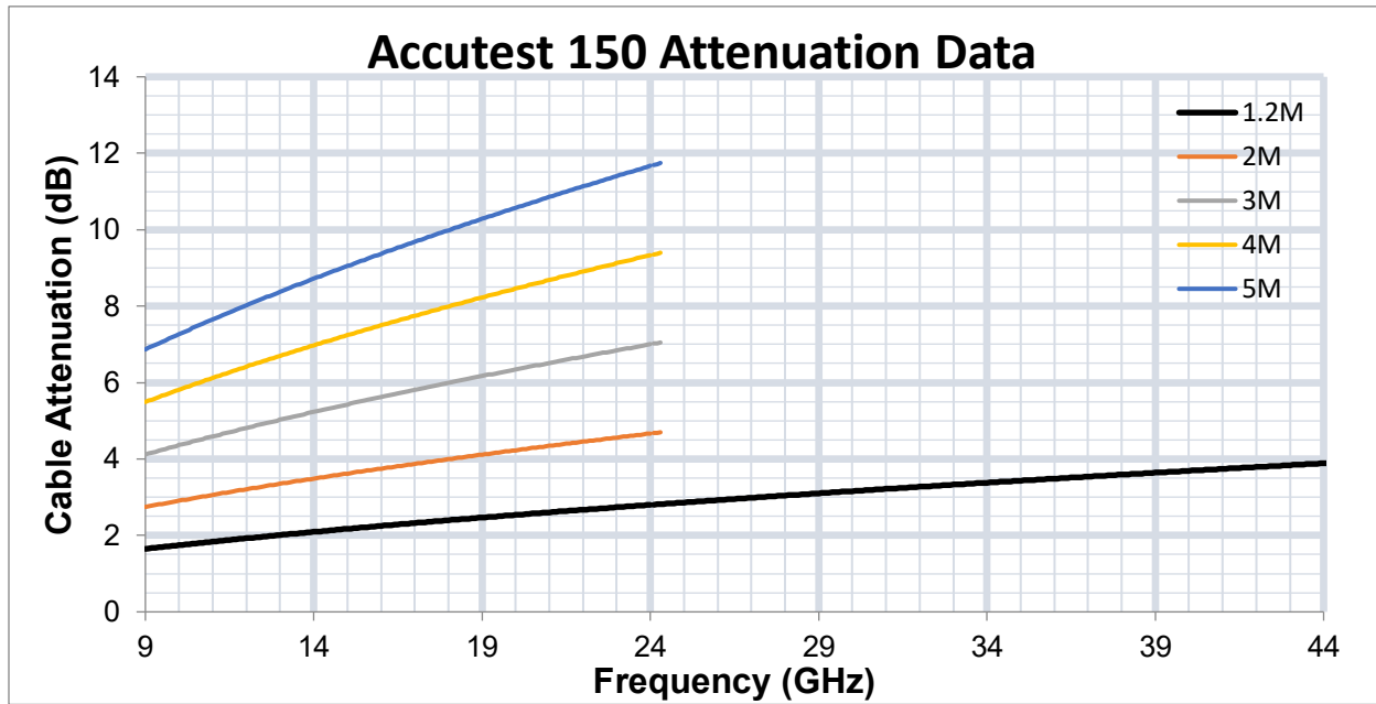
FIGURE 16: INSERTION LOSS OF ACCUTEST 150 (RF/LO CABLE) WITH RESPECT TO FREQUENCY. THIS CHART CAN BE USED TO CALCULATE CABLE LOSSES IN YOUR SYSTEM
