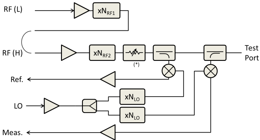
FIGURE 4: TxRx BLOCK DIAGRAM: WM164 (STANDARD SIZE)
