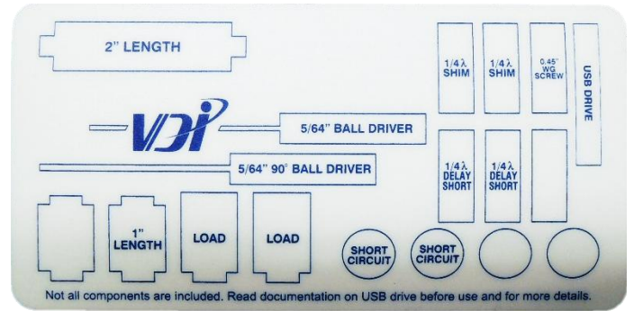
FIGURE 11: TYPE B TRL CALIBRATION KIT
