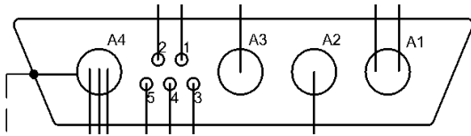
VDI-175 Output Connector shown
