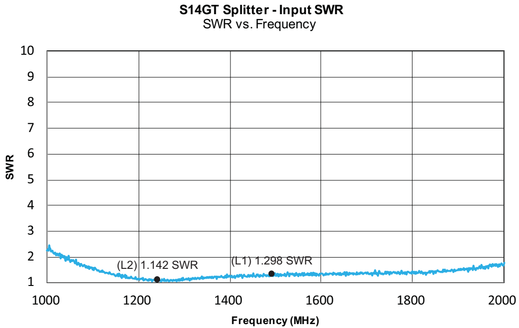
Figure 2-2. Input SWR (10dB)
