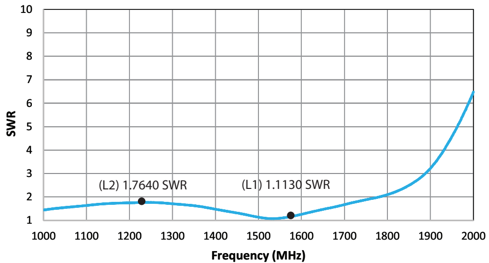
Figure 2-2. SWR vs. Frequency
